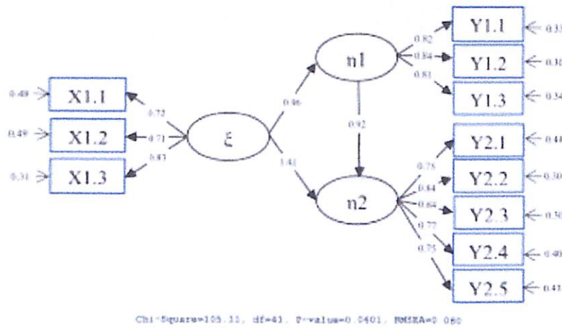
Gambar 16 Diagram Jalur full model antar variabel
